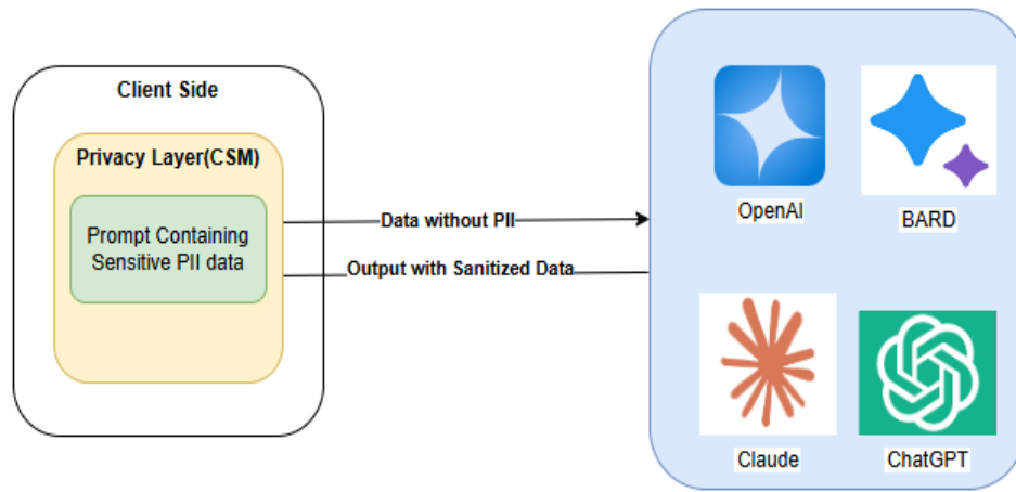
Figure 1.0.3 PII Data with CSM Privacy Layer
