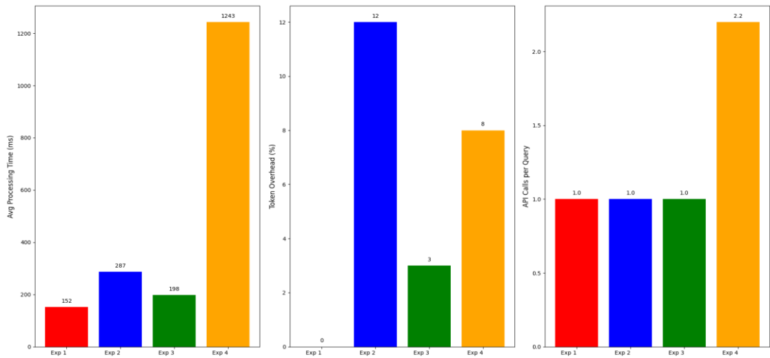
Figure 5.0.4 Experiment 1,2,3,4 Computational Efficiency Metrics
