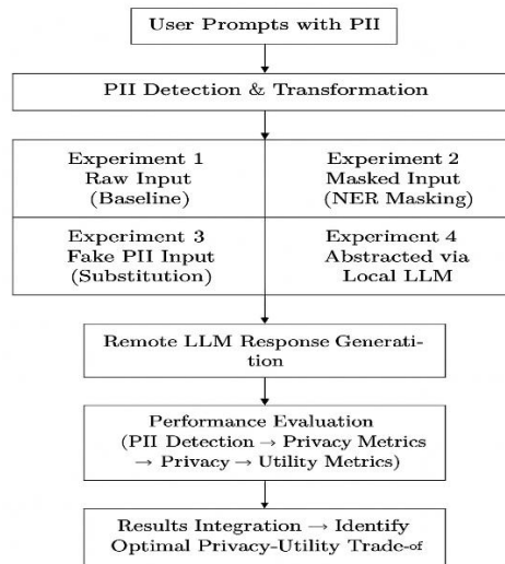
Figure 3.0.1 Steps in Experimental set-up for Privacy–Utility Data Preparation
