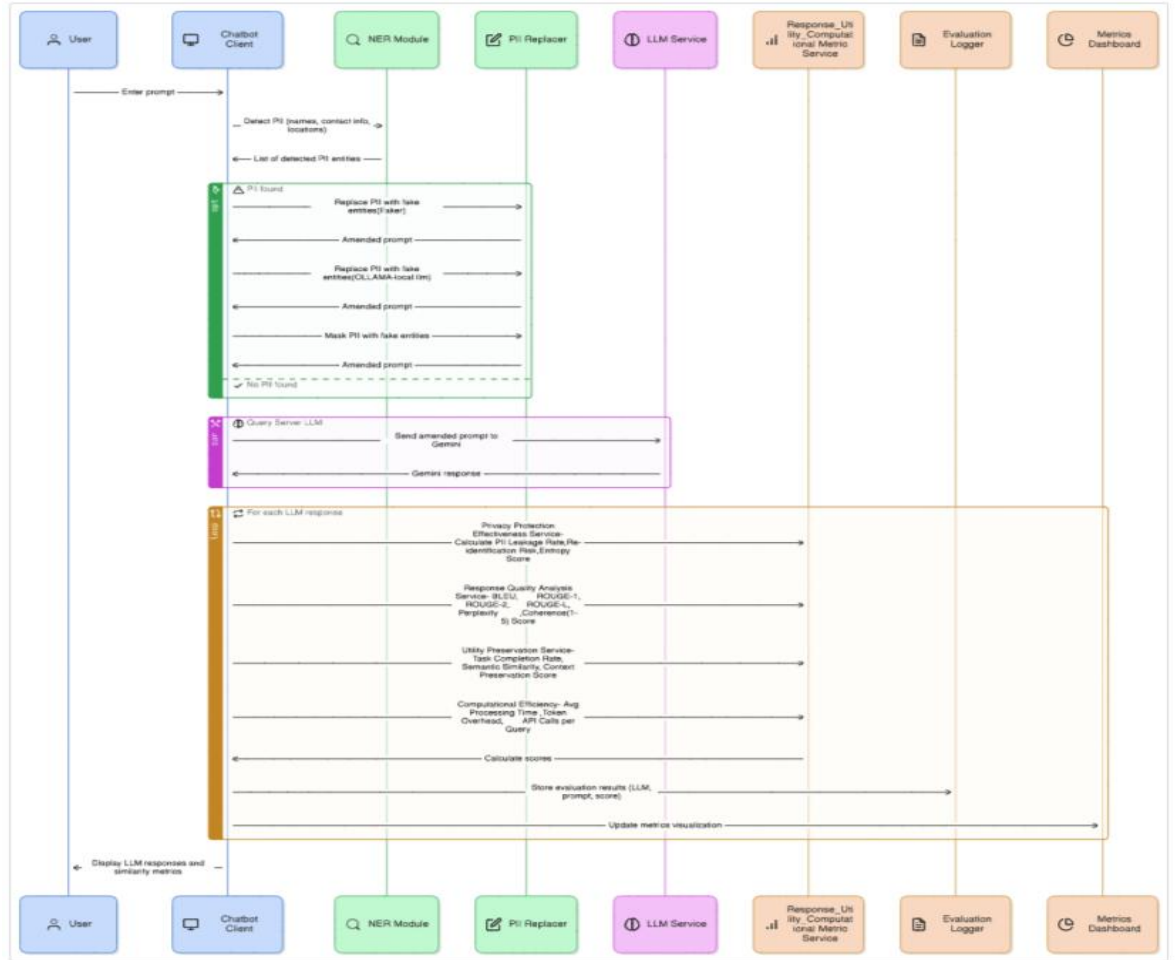
Figure 3.0.2 Interaction Diagram for CSM
