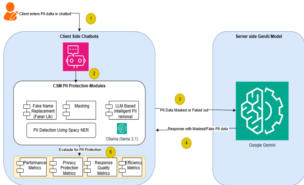
Figure 4.0.1 Explaining various components in Architecture
