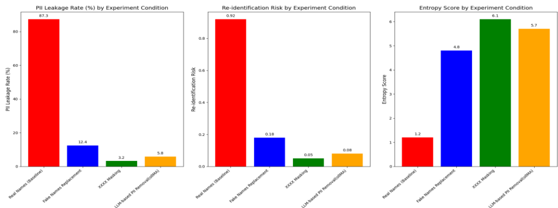
Figure 5.0.1 Experiment 1,2,3,4 Privacy Protection Metrics Results
