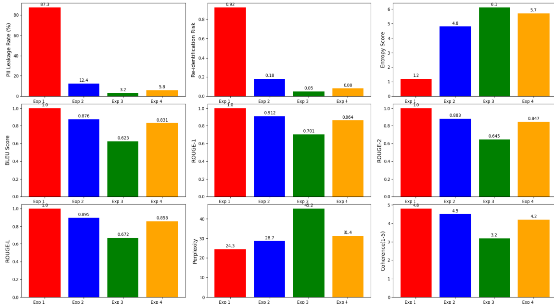
Figure 5.0.2 Experiment 1,2,3,4 Response Quality Analysis
